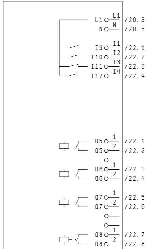
LOGO Modul DM8 230R 4x INPUT / 4x RELAY OUTPUT
