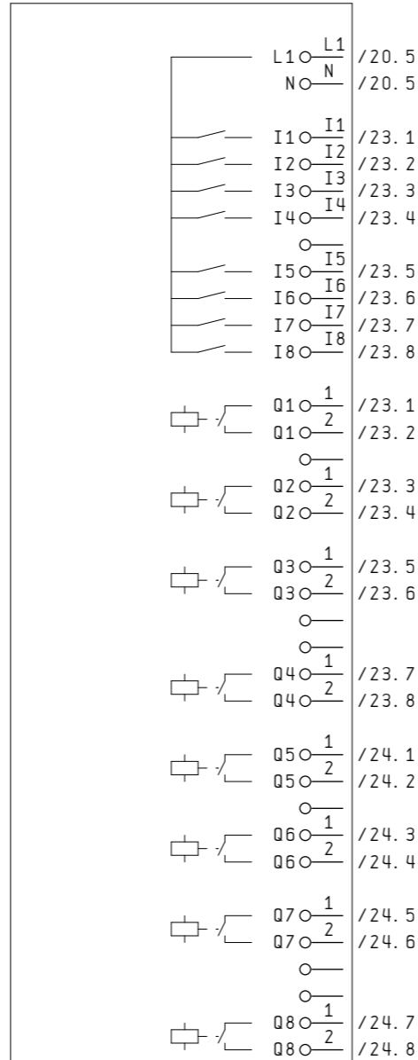
LOGO Modul DM16 230R 8x INPUT / 8x RELAY OUTPUT
