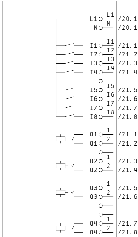
LOGO Modul 230RC 8x INPUT / 4x RELAY OUTPUT
