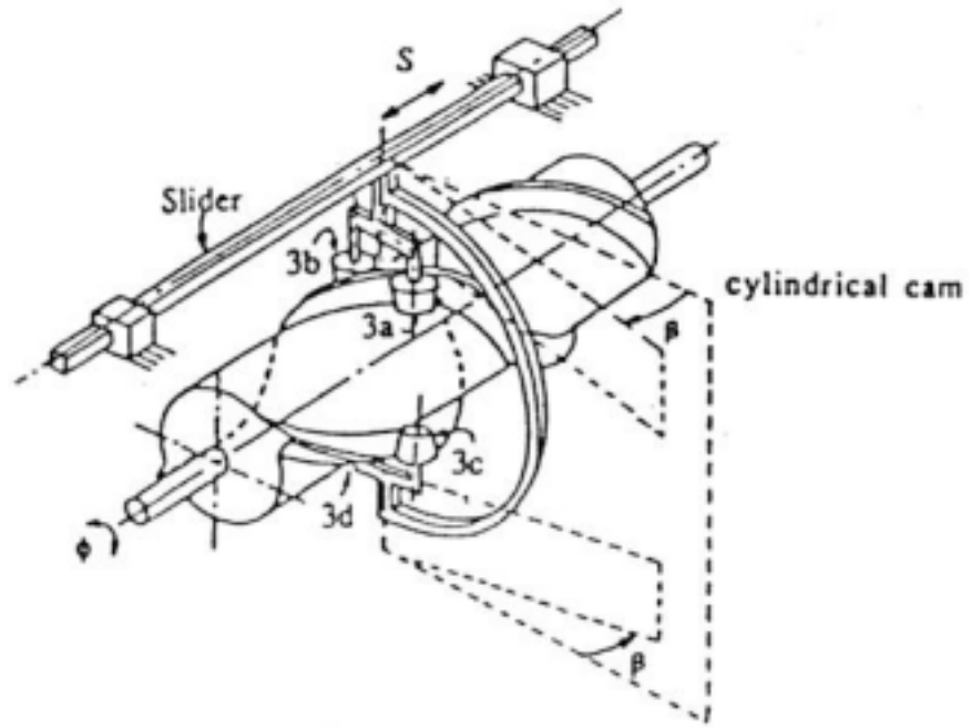
Fig. 2.7 A cylindrical conjugate cam with a translating follower
