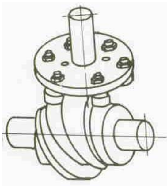
Fig.2.10 Cylindrical conjugate cams with a rotating roller gear (follower)
