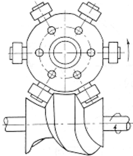
Fig.2.9 Cylindrical conjugate cams with a rotating roller gear (follower)
