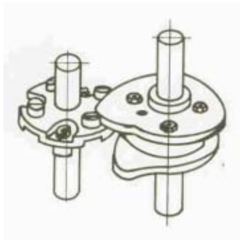
Fig. 2.8 Double-disk conjugate cams with a rotating roller gear (follower)
