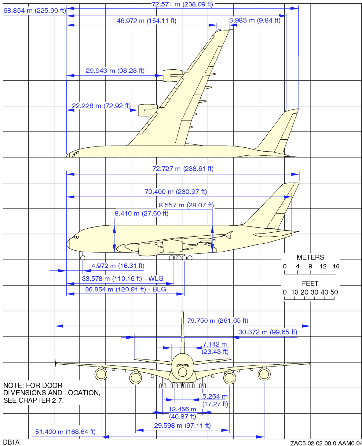
General Airplane Dimensions A380-800/800F Models
