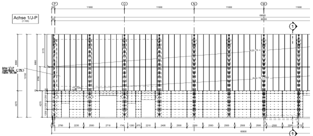
Kassette Achse 1 1:100 Kassette 100x50-C-68
